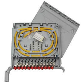
Optical Splice & Distribution Module Series F (F1 F2)
